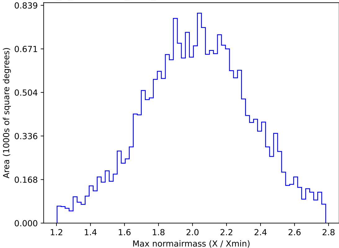
early_u_fpextra3.0_v3.4_10yrs All sky y band: Max normairmass
