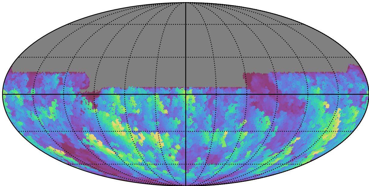
early_u_fpextra3.0_v3.4_10yrs All sky u band: Max normairmass
