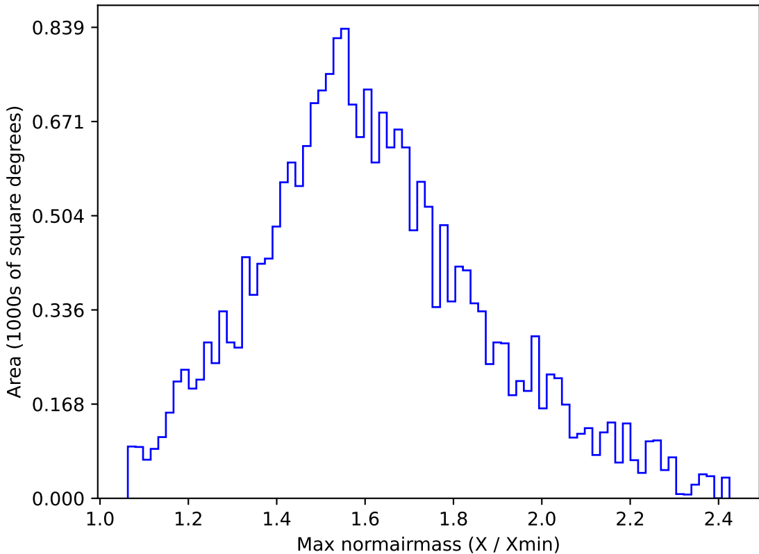
early_u_fpextra3.0_v3.4_10yrs All sky u band: Max normairmass
