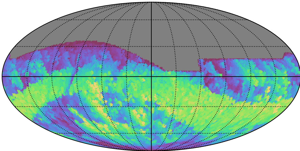
early_u_fpextra3.0_v3.4_10yrs All sky r band: Max normairmass
