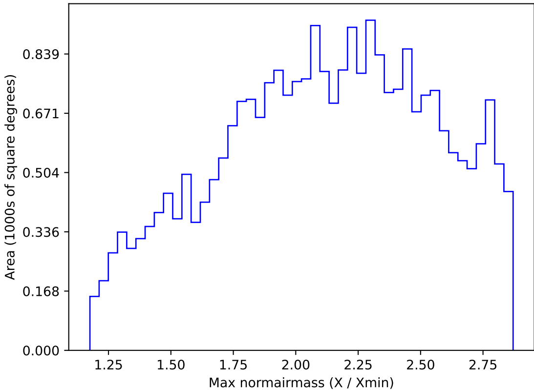
early_u_fpextra3.0_v3.4_10yrs All sky i band: Max normairmass
