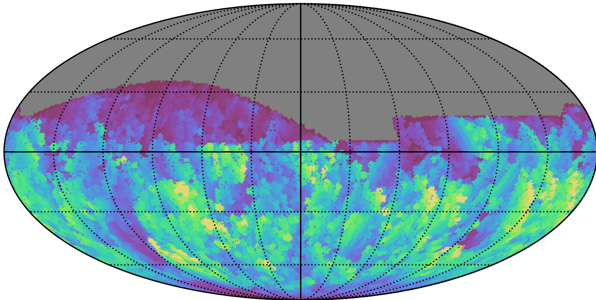
early_u_fpextra3.0_v3.4_10yrs All sky g band: Max normairmass
