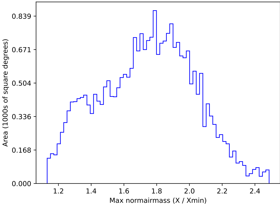
early_u_fpextra3.0_v3.4_10yrs All sky g band: Max normairmass
