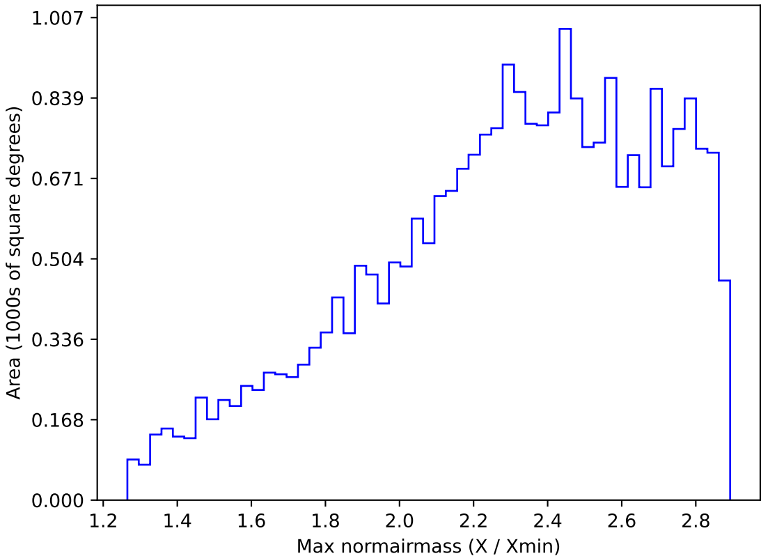
early_u_fpextra3.0_v3.4_10yrs All sky all bands: Max normairmass
