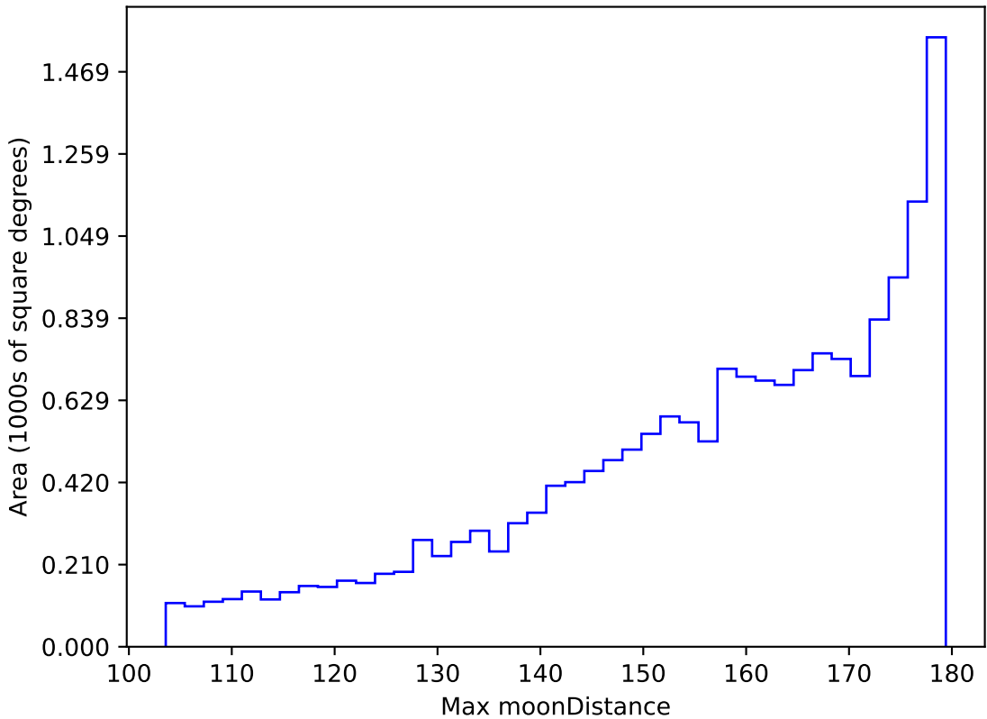
early_u_fpextra3.0_v3.4_10yrs WFD r band: Max moonDistance
