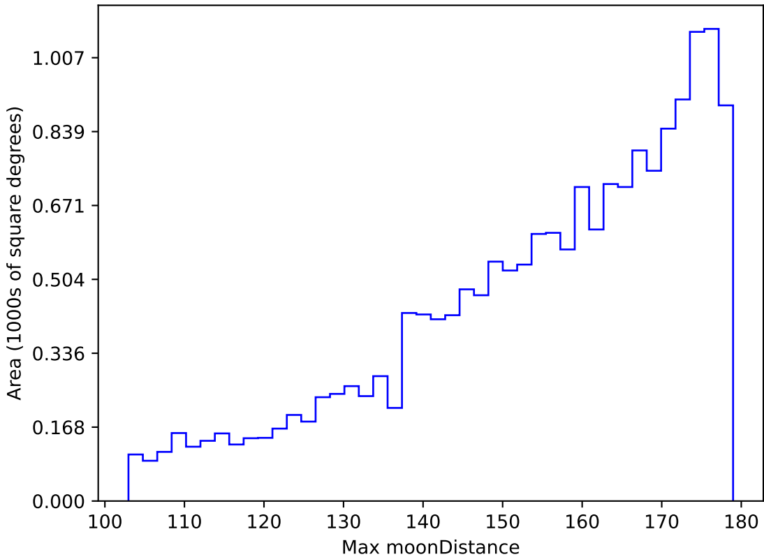
early_u_fpextra3.0_v3.4_10yrs WFD g band: Max moonDistance
