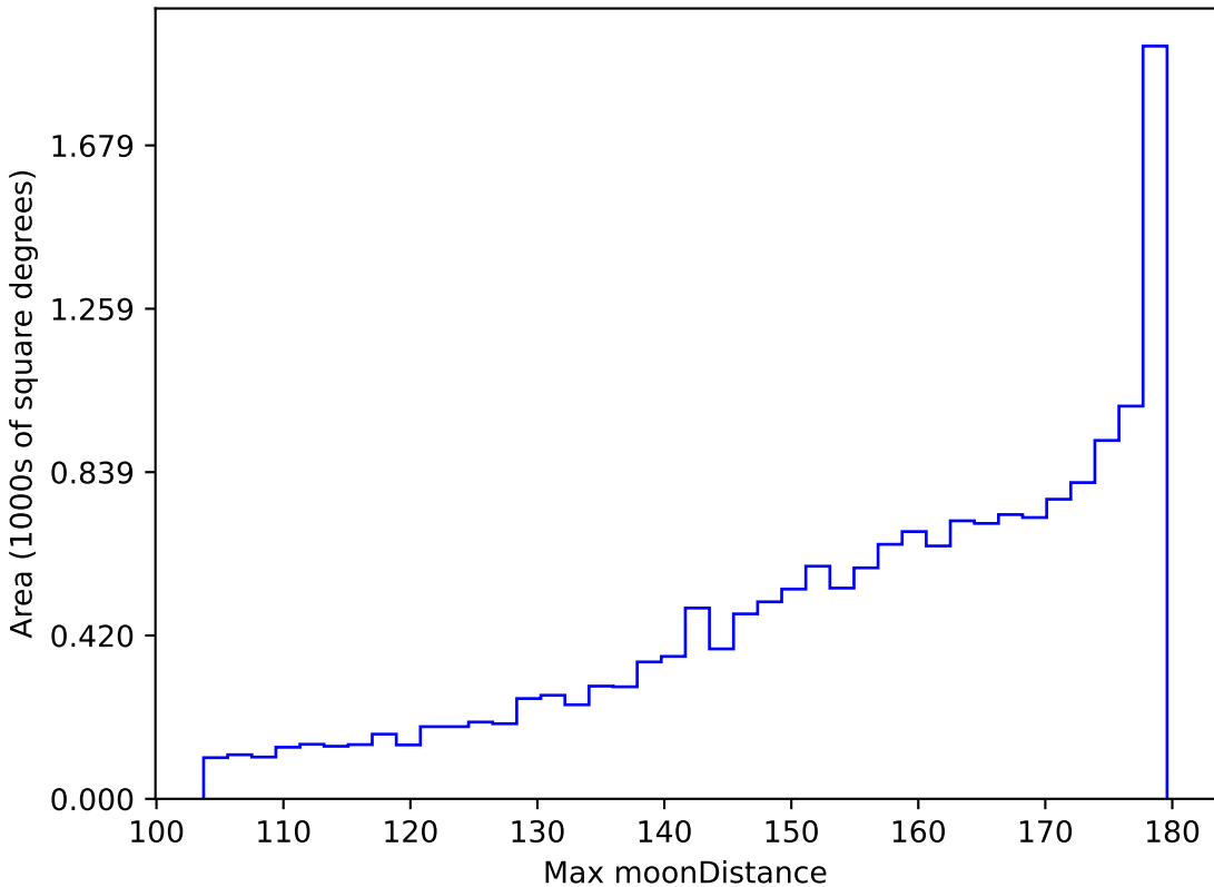
early_u_fpextra3.0_v3.4_10yrs WFD all bands: Max moonDistance
