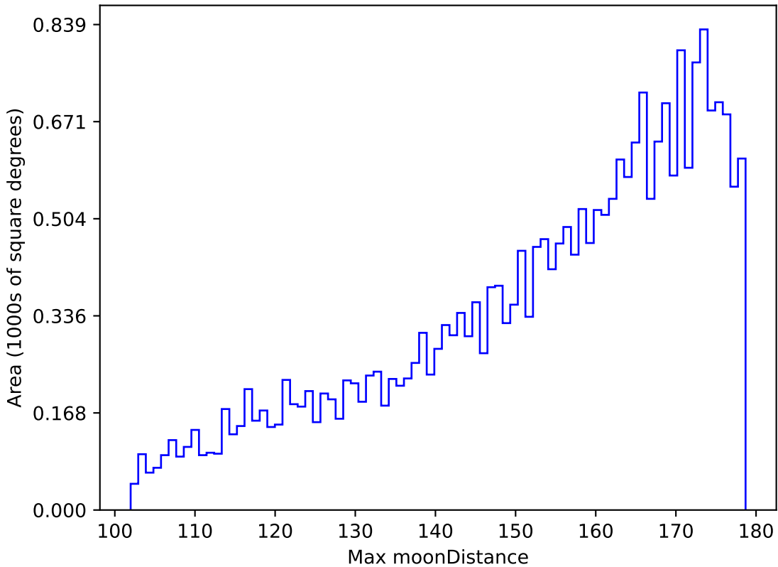
early_u_fpextra3.0_v3.4_10yrs All sky z band: Max moonDistance
