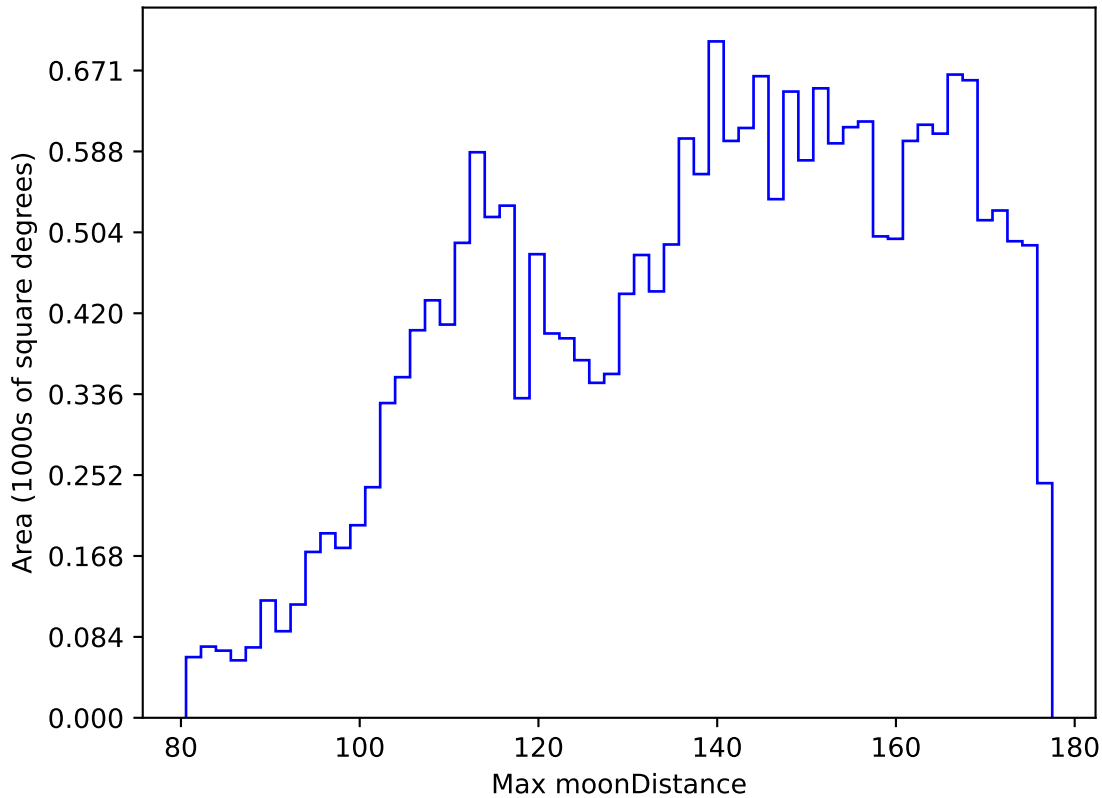
early_u_fpextra3.0_v3.4_10yrs All sky y band: Max moonDistance
