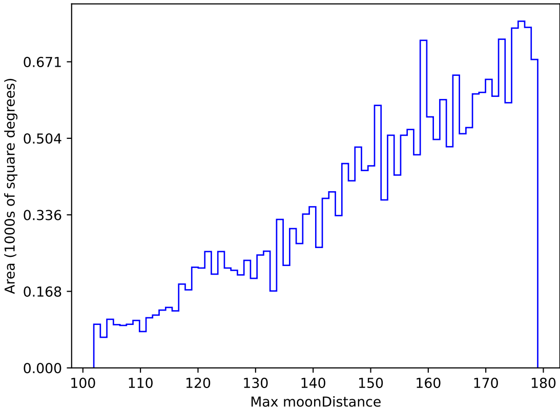
early_u_fpextra3.0_v3.4_10yrs All sky u band: Max moonDistance
