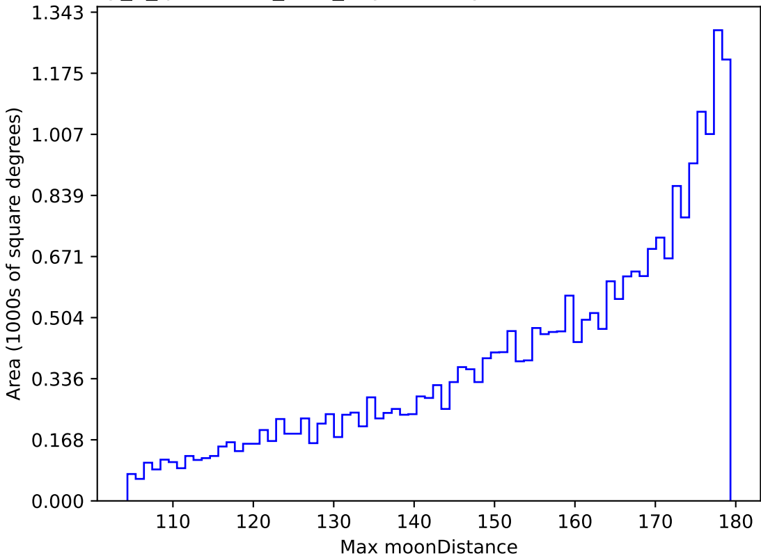
early_u_fpextra3.0_v3.4_10yrs All sky r band: Max moonDistance
