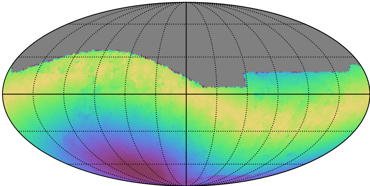
early_u_fpextra3.0_v3.4_10yrs All sky i band: Max moonDistance
