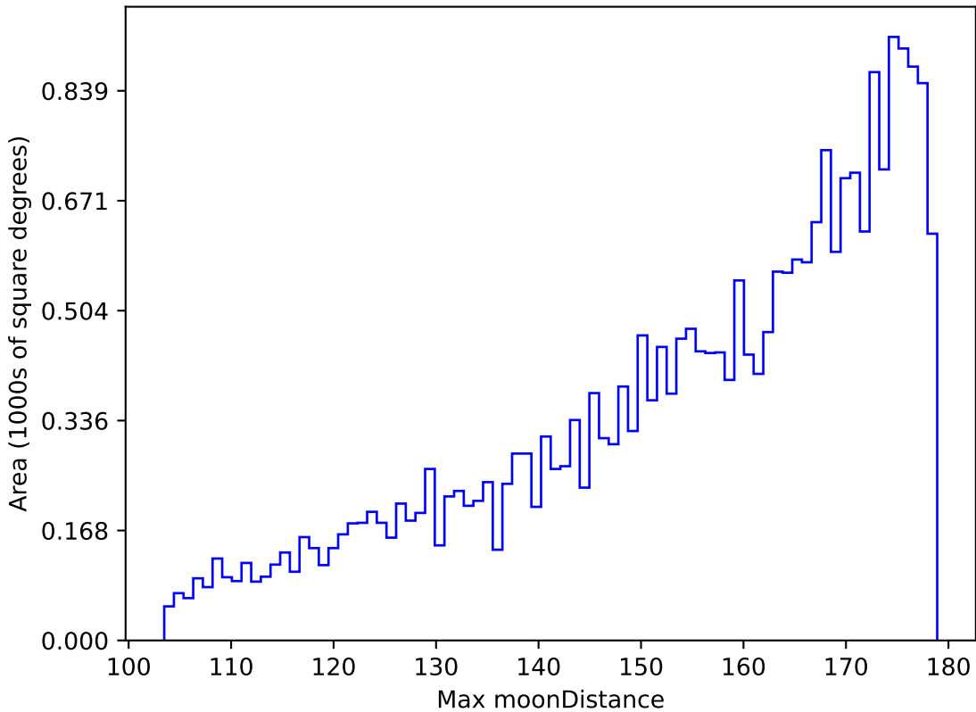
early_u_fpextra3.0_v3.4_10yrs All sky g band: Max moonDistance
