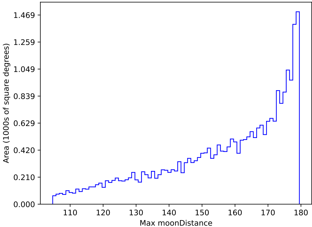
early_u_fpextra3.0_v3.4_10yrs All sky all bands: Max moonDistance
