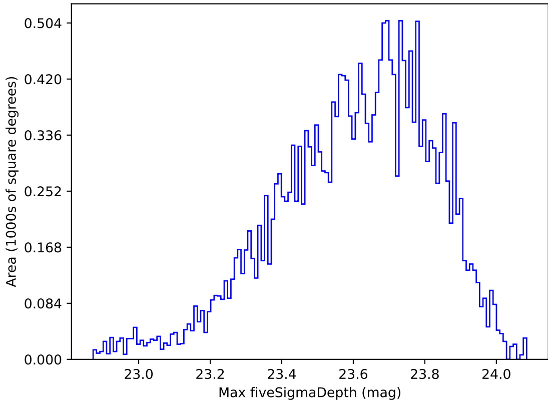
early_u_fpextra3.0_v3.4_10yrs Yr 1 u band: Max fiveSigmaDepth
