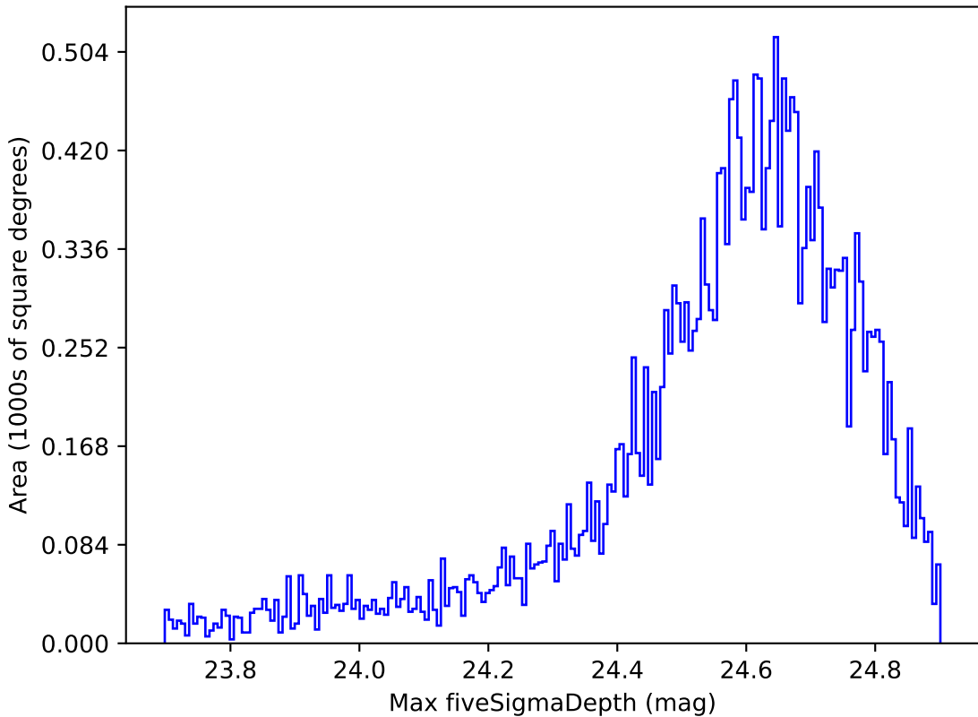
early_u_fpextra3.0_v3.4_10yrs Yr 1 r band: Max fiveSigmaDepth
