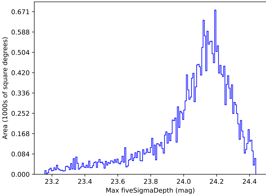
early_u_fpextra3.0_v3.4_10yrs Yr 1 i band: Max fiveSigmaDepth
