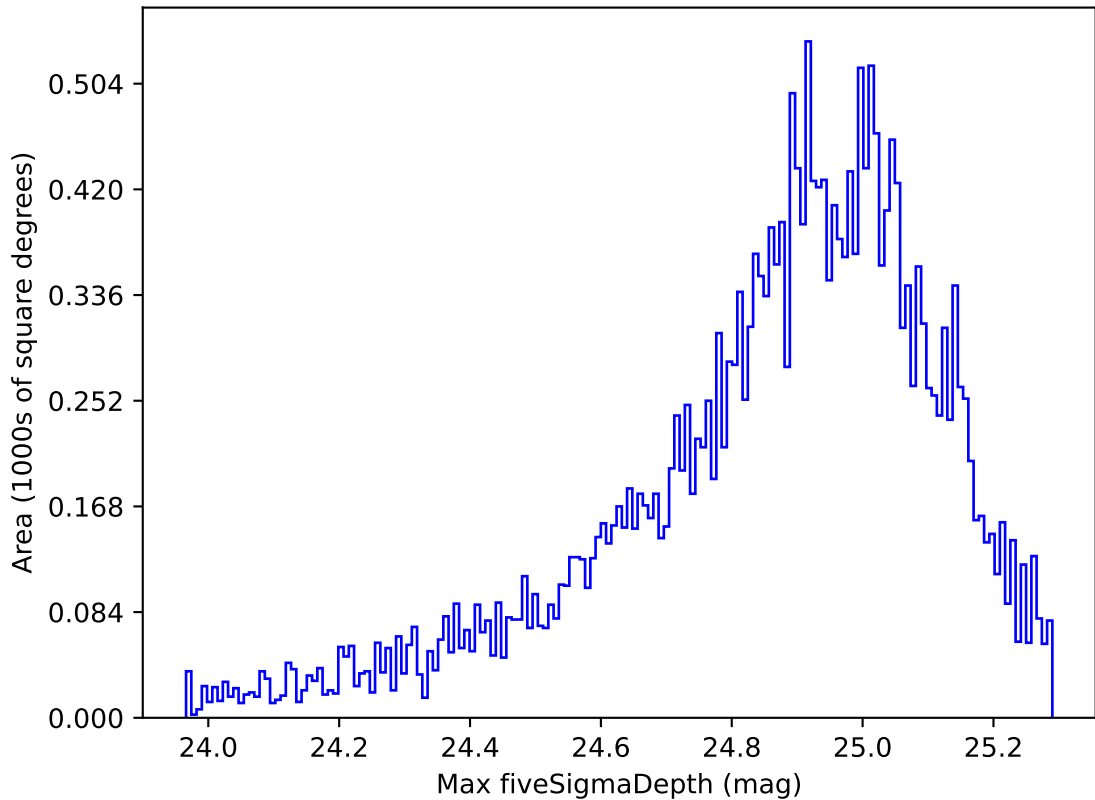
early_u_fpextra3.0_v3.4_10yrs Yr 1 g band: Max fiveSigmaDepth
