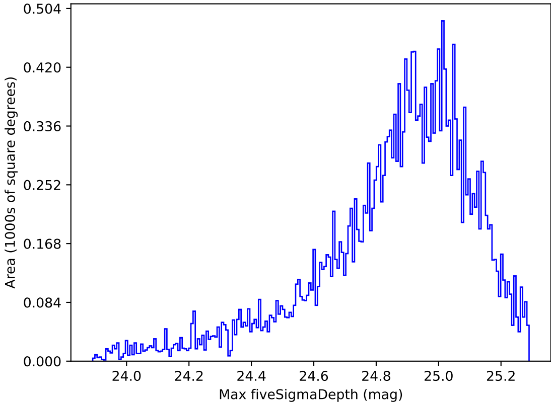
early_u_fpextra3.0_v3.4_10yrs Yr 1 all bands: Max fiveSigmaDepth
