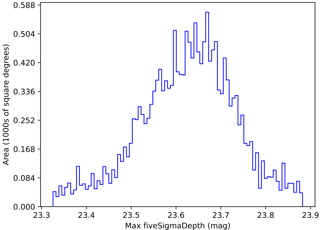
early_u_fpextra3.0_v3.4_10yrs WFD z band: Max fiveSigmaDepth
