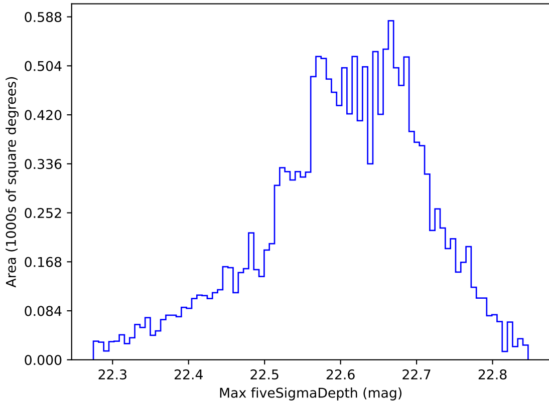
early_u_fpextra3.0_v3.4_10yrs WFD y band: Max fiveSigmaDepth
