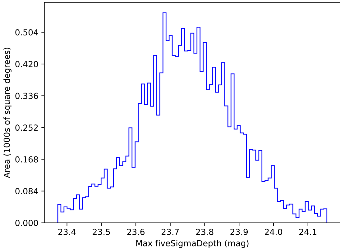
early_u_fpextra3.0_v3.4_10yrs WFD u band: Max fiveSigmaDepth
