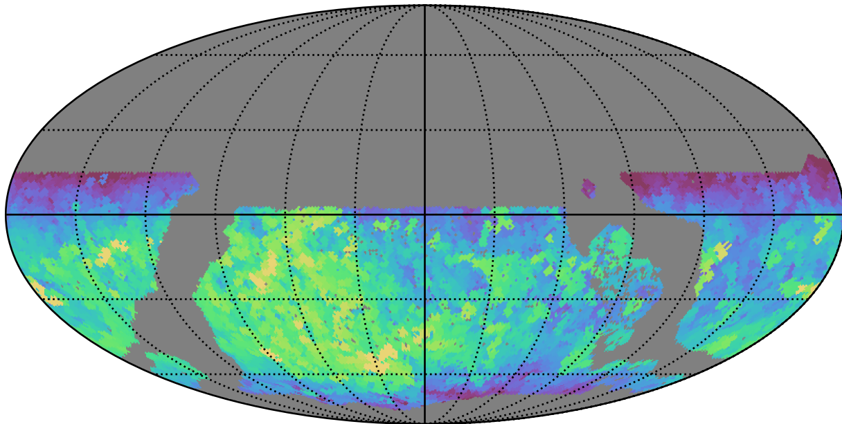
early_u_fpextra3.0_v3.4_10yrs WFD r band: Max fiveSigmaDepth
