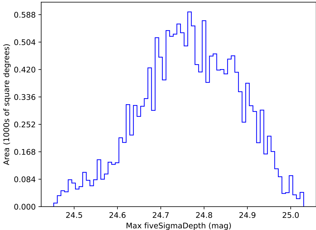
early_u_fpextra3.0_v3.4_10yrs WFD r band: Max fiveSigmaDepth
