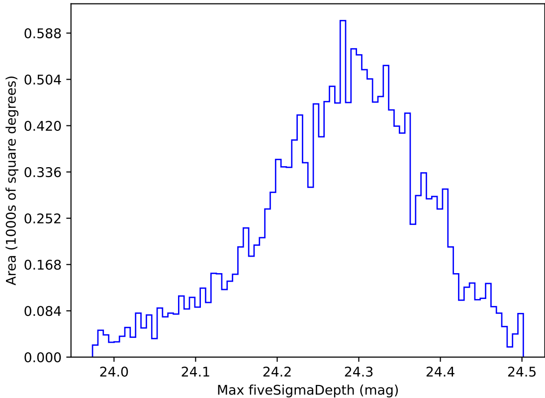
early_u_fpextra3.0_v3.4_10yrs WFD i band: Max fiveSigmaDepth
