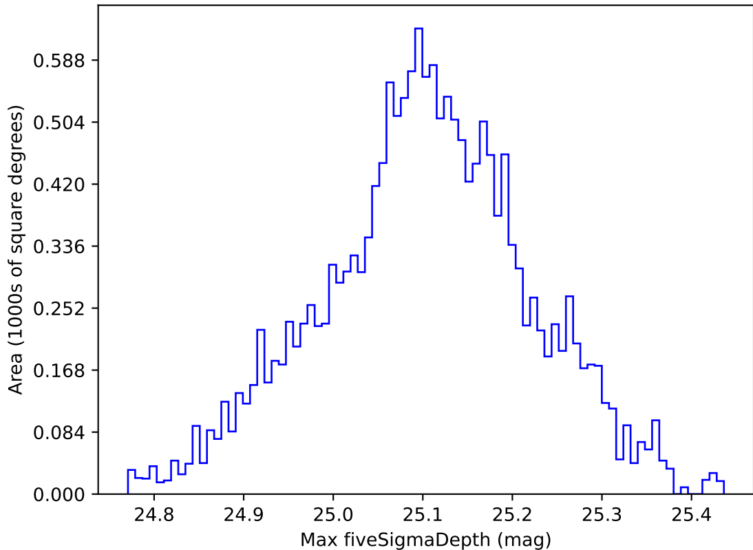
early_u_fpextra3.0_v3.4_10yrs WFD g band: Max fiveSigmaDepth
