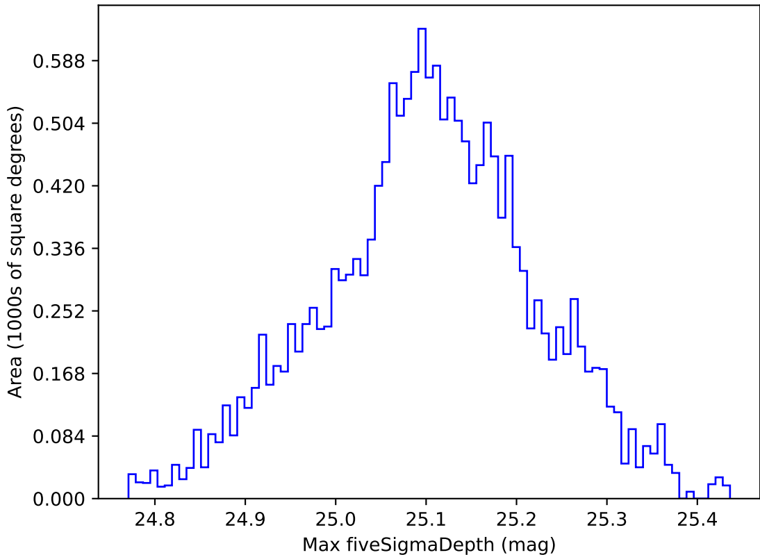
early_u_fpextra3.0_v3.4_10yrs WFD all bands: Max fiveSigmaDepth
