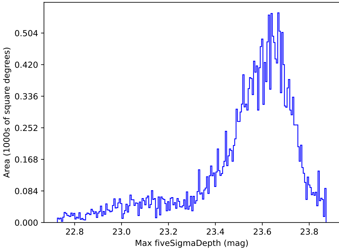
early_u_fpextra3.0_v3.4_10yrs All sky z band: Max fiveSigmaDepth
