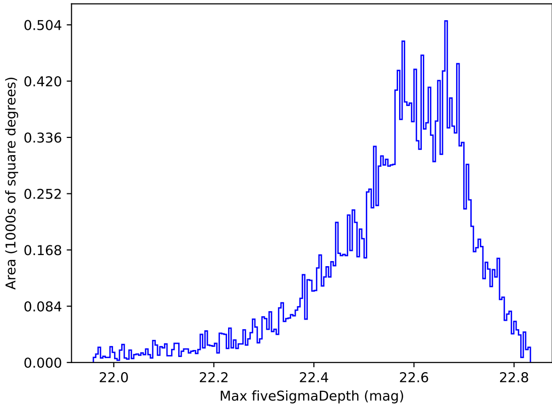
early_u_fpextra3.0_v3.4_10yrs All sky y band: Max fiveSigmaDepth
