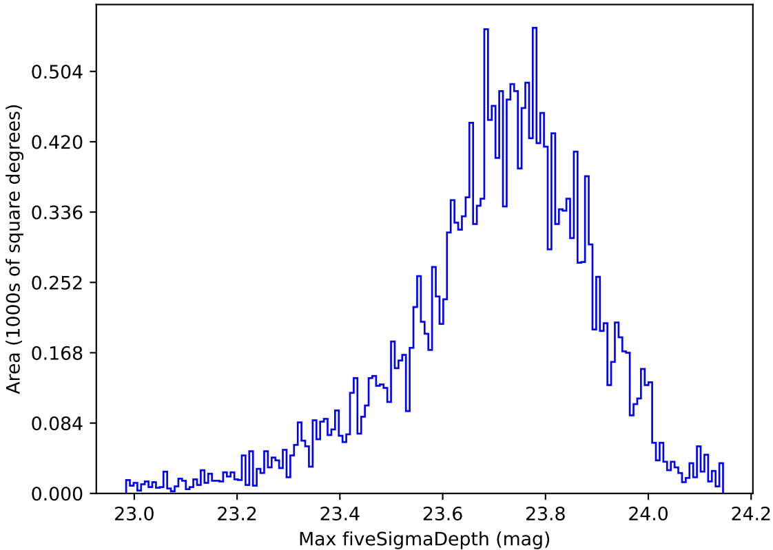
early_u_fpextra3.0_v3.4_10yrs All sky u band: Max fiveSigmaDepth
