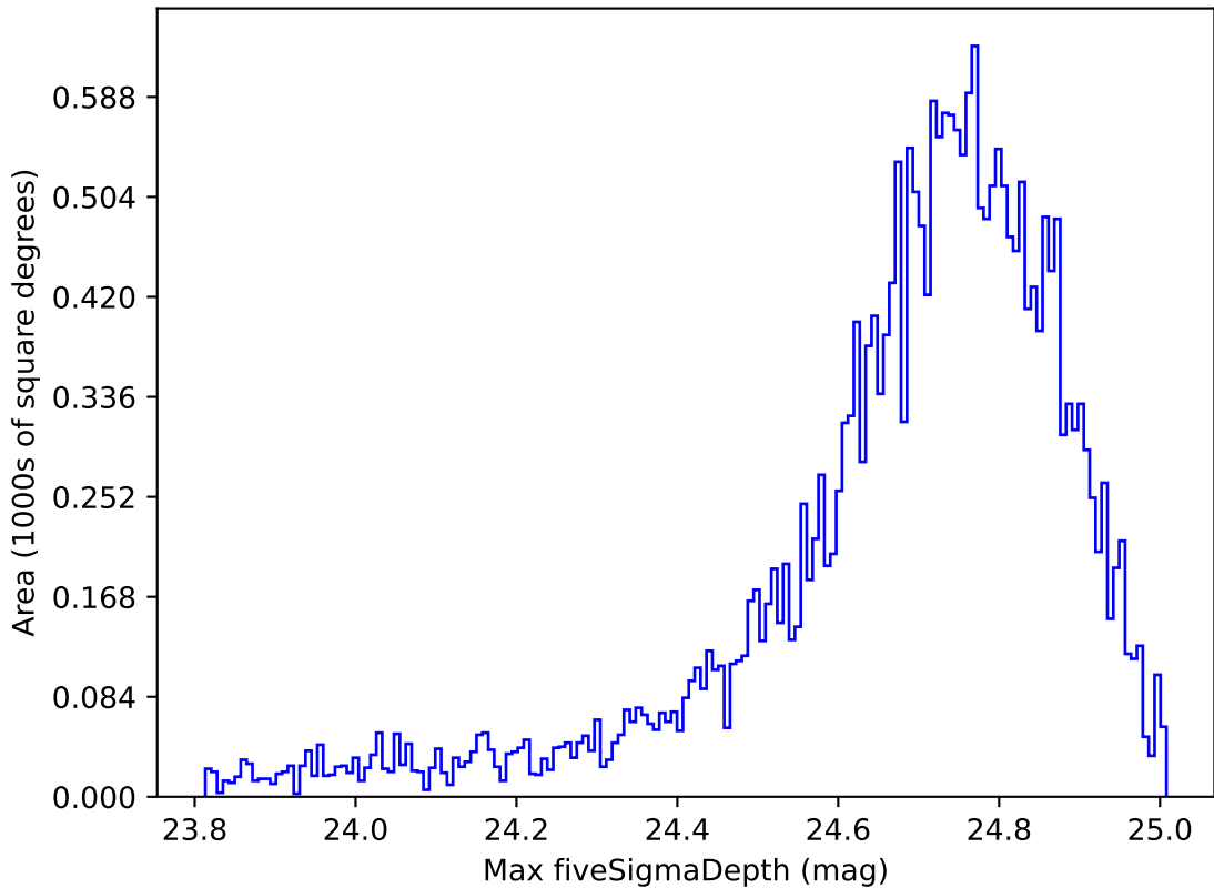
early_u_fpextra3.0_v3.4_10yrs All sky r band: Max fiveSigmaDepth
