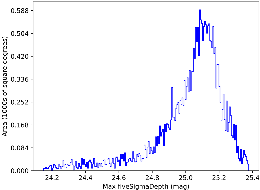
early_u_fpextra3.0_v3.4_10yrs All sky g band: Max fiveSigmaDepth
