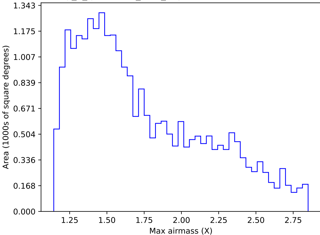
early_u_fpextra3.0_v3.4_10yrs Yr 1 z band: Max airmass
