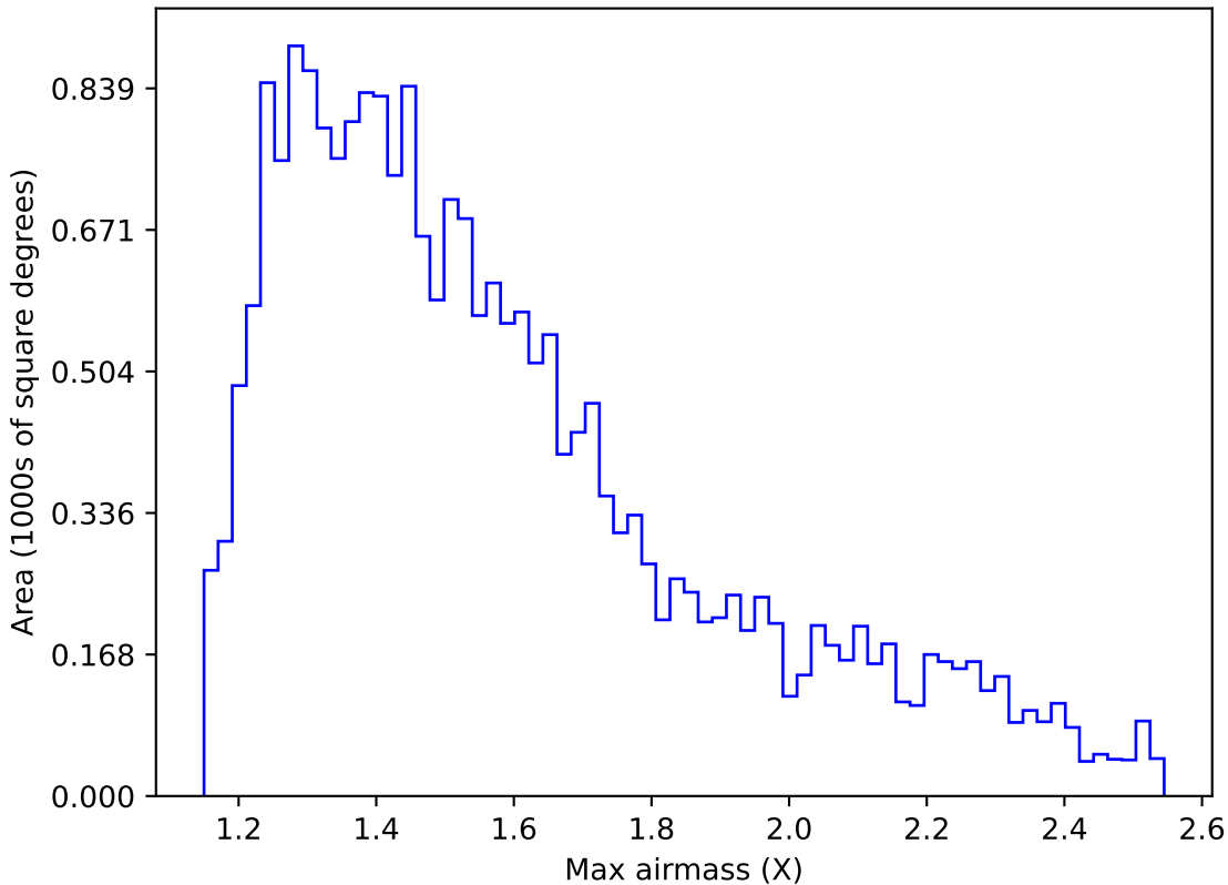
early_u_fpextra3.0_v3.4_10yrs Yr 1 y band: Max airmass
