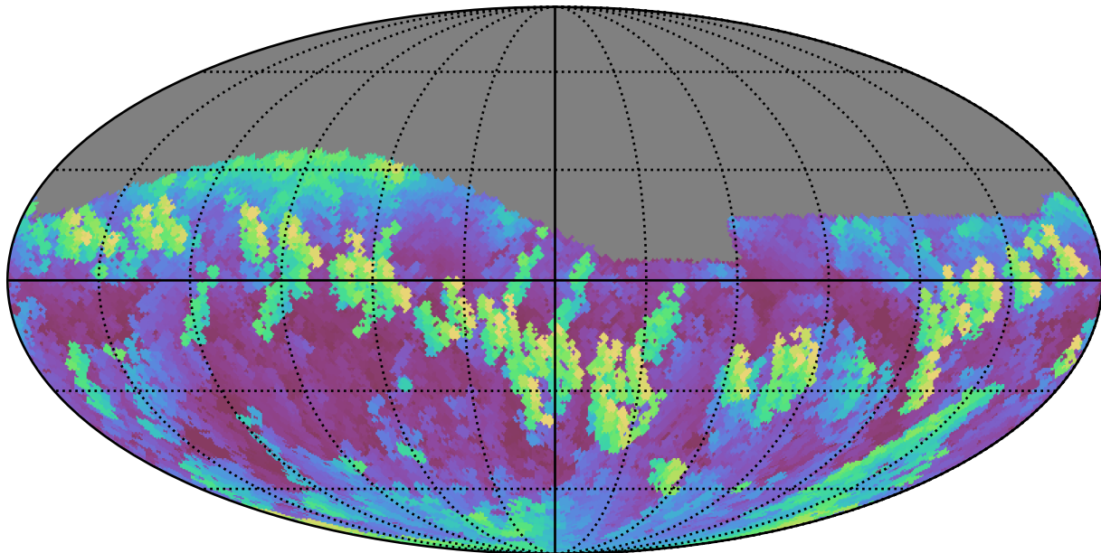
early_u_fpextra3.0_v3.4_10yrs Yr 1 i band: Max airmass
