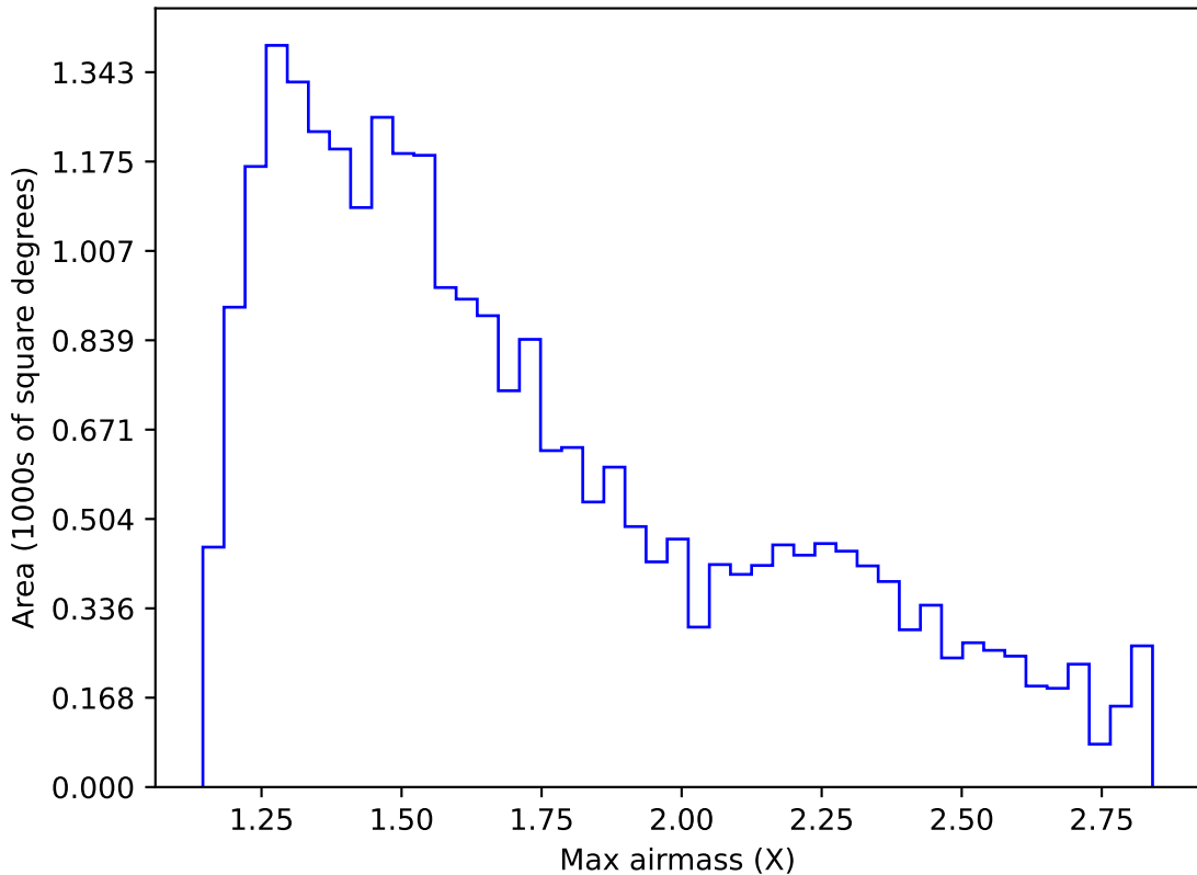
early_u_fpextra3.0_v3.4_10yrs Yr 1 i band: Max airmass
