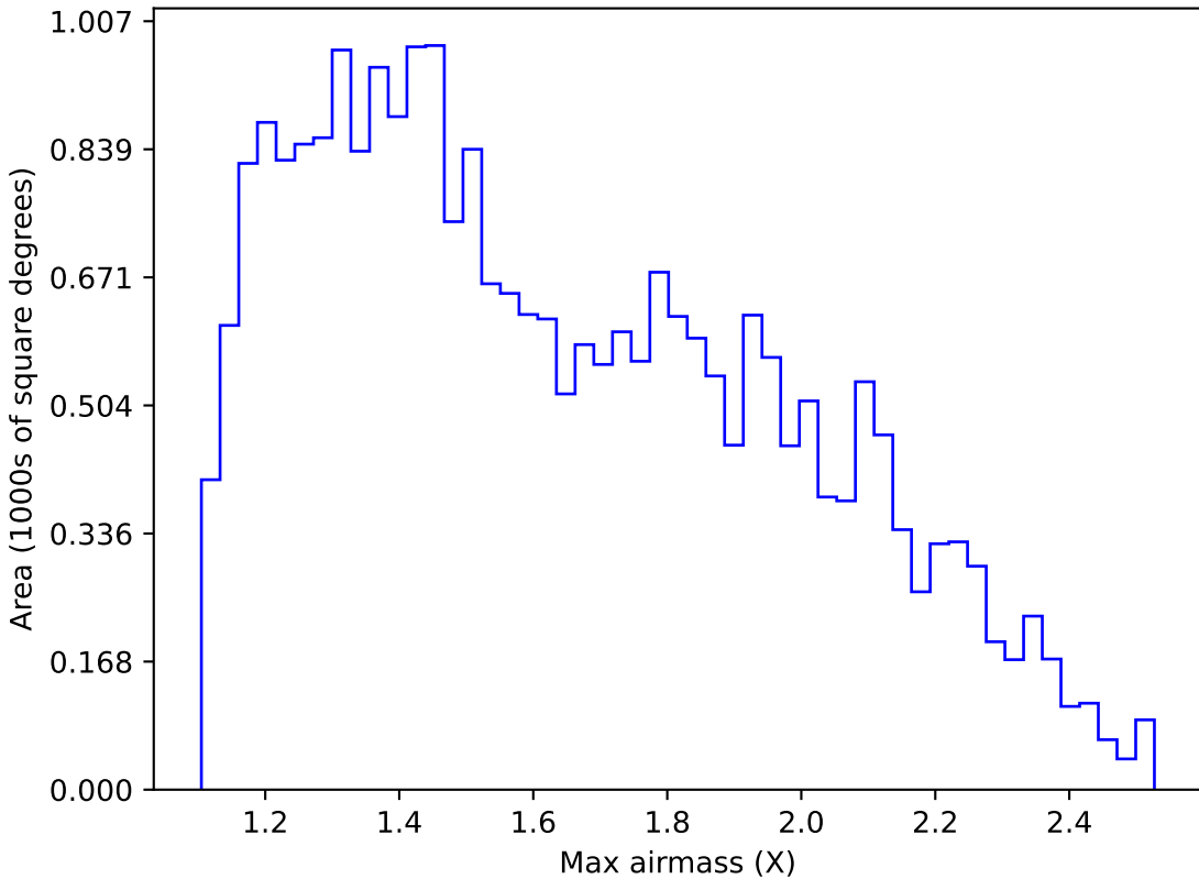
early_u_fpextra3.0_v3.4_10yrs Yr 1 g band: Max airmass
