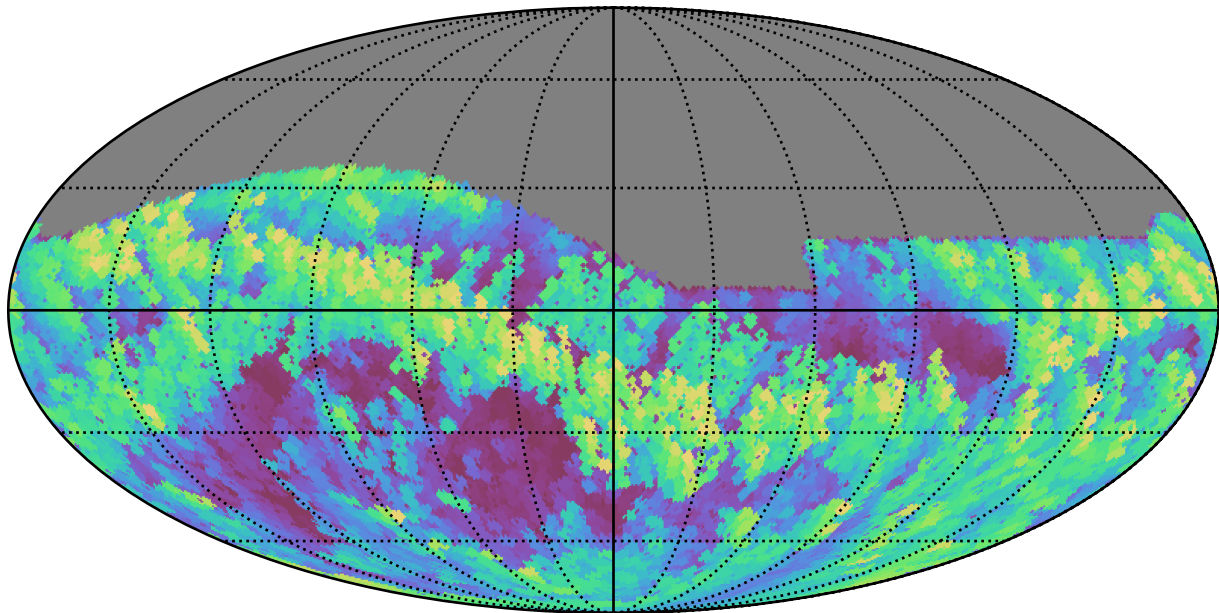
early_u_fpextra3.0_v3.4_10yrs Yr 1 all bands: Max airmass
