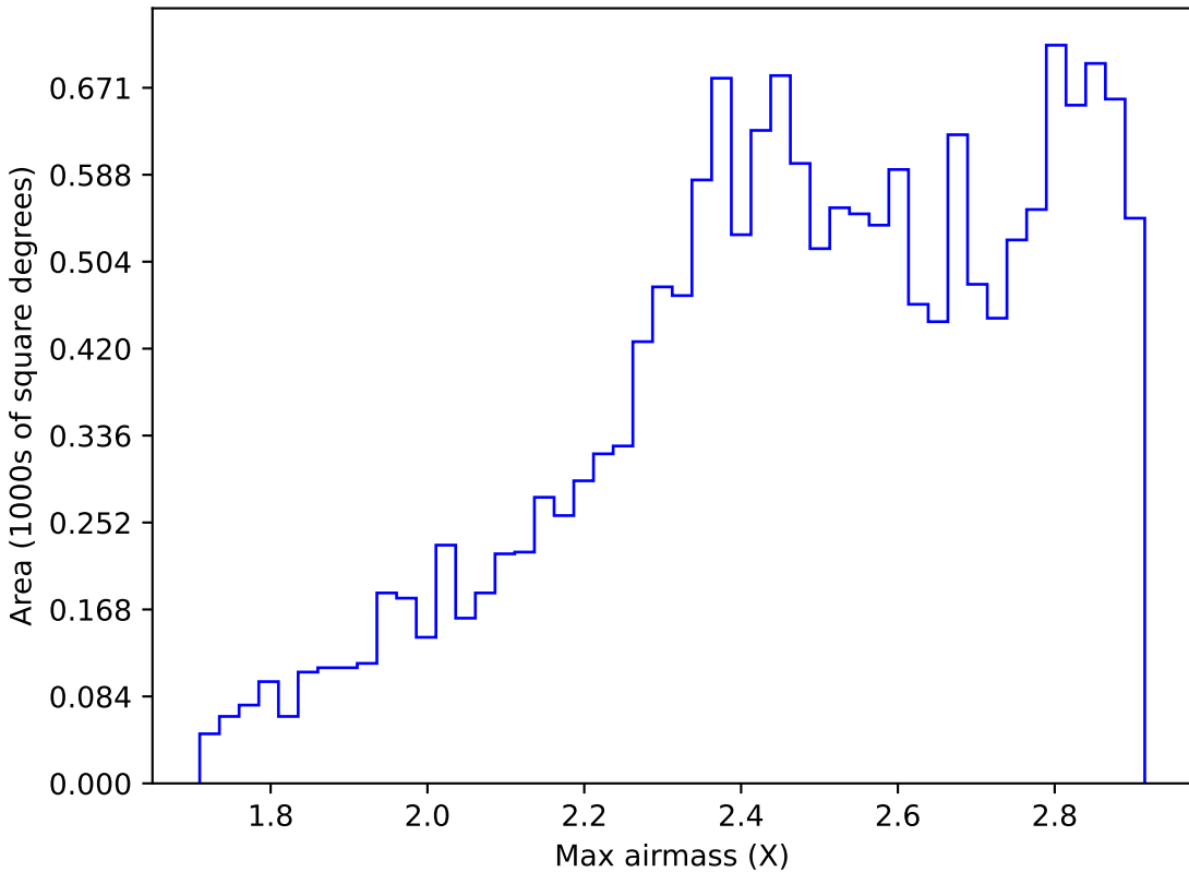
early_u_fpextra3.0_v3.4_10yrs WFD z band: Max airmass
