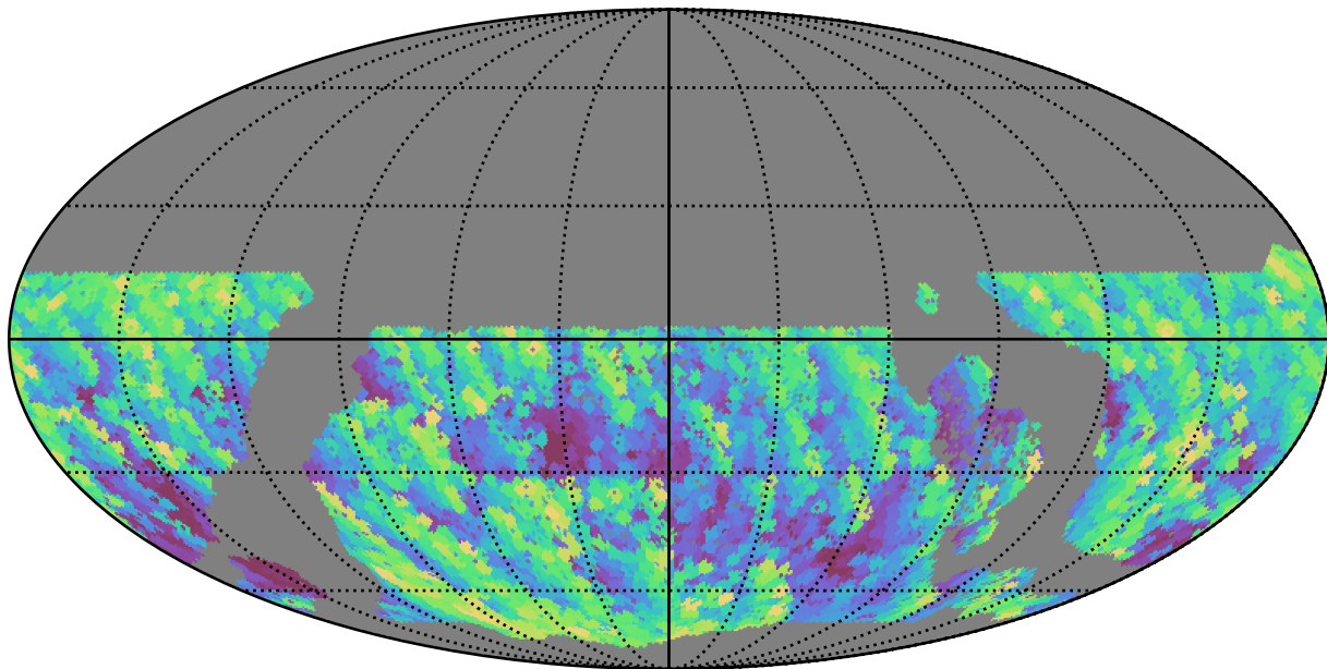
early_u_fpextra3.0_v3.4_10yrs WFD y band: Max airmass
