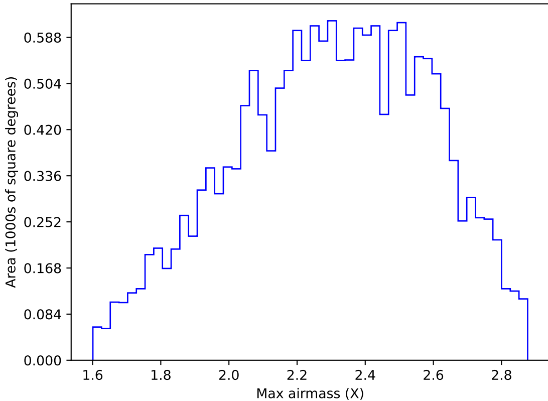
early_u_fpextra3.0_v3.4_10yrs WFD y band: Max airmass
