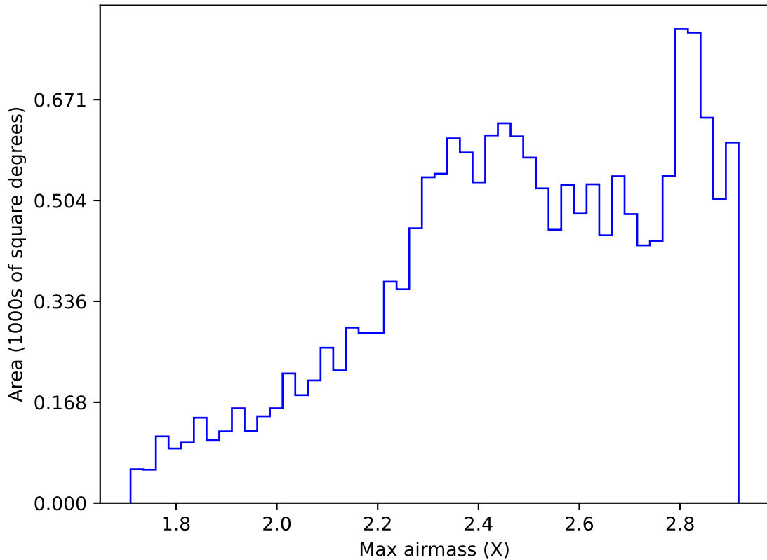
early_u_fpextra3.0_v3.4_10yrs WFD i band: Max airmass
