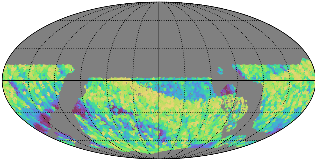
early_u_fpextra3.0_v3.4_10yrs WFD all bands: Max airmass
