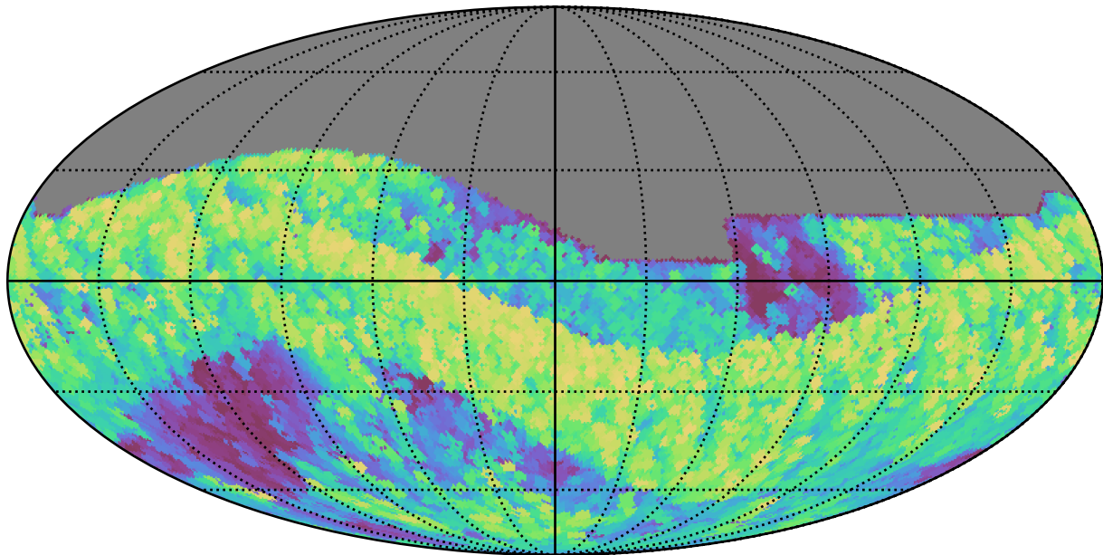
early_u_fpextra3.0_v3.4_10yrs All sky z band: Max airmass
