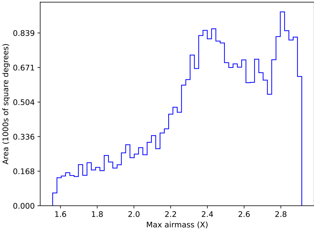
early_u_fpextra3.0_v3.4_10yrs All sky z band: Max airmass
