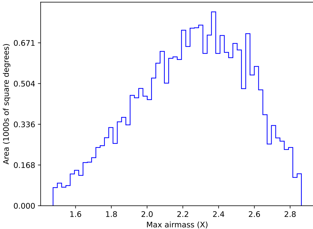
early_u_fpextra3.0_v3.4_10yrs All sky y band: Max airmass
